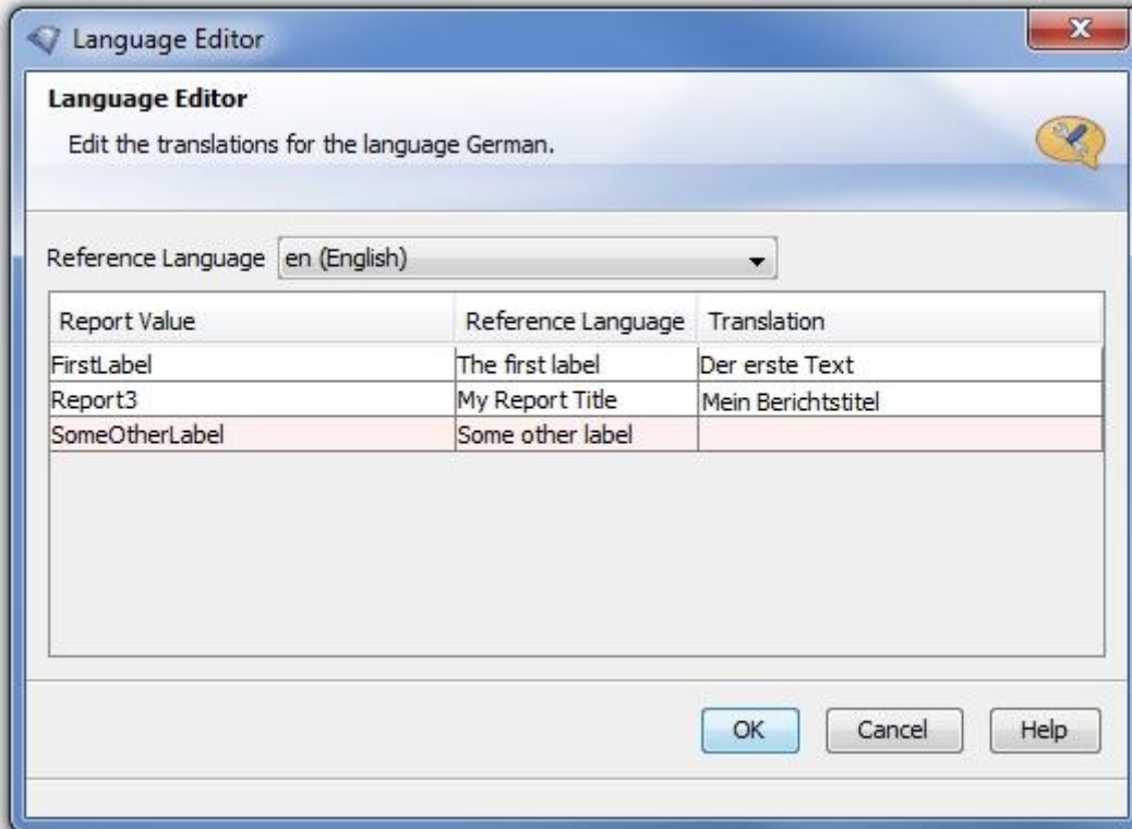
Fig. 2: Language Editor
